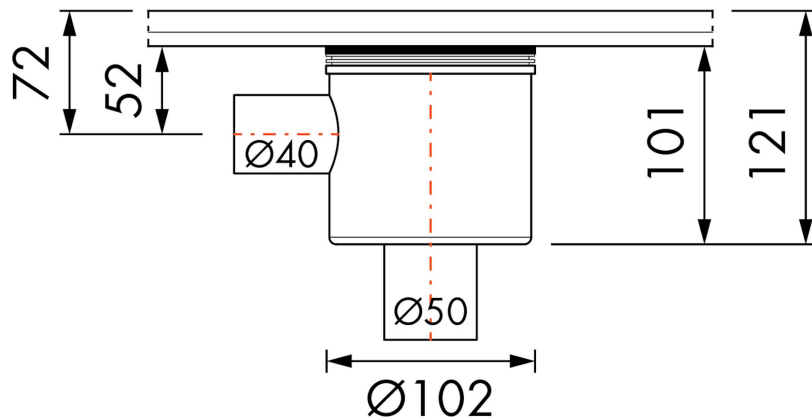
Easy Drain® EDMSI-4, WS-50 mm
